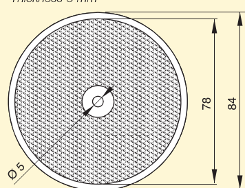
CT80-RFL000008 Spessore 8 mm Thickness 8 mm
