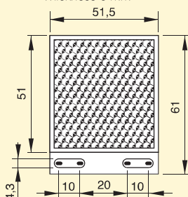
CTR8-RFL000017 Spessore 8 mm Thickness 8 mm
