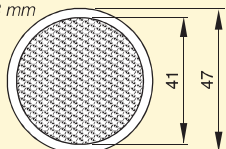
CTR2-RFL000013 Spessore 5 mm Thickness 5 mm
