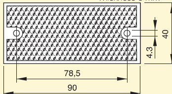
CTR2-RFL000013 Spessore 5 mm Thickness 5 mm
