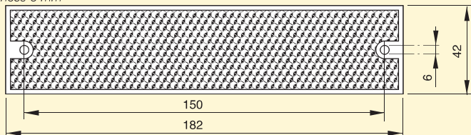
CTR8-RFL000017 Spessore 8 mm Thickness 8 mm
